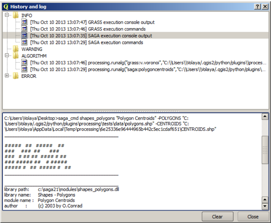
Figure 17.3: Processing History
