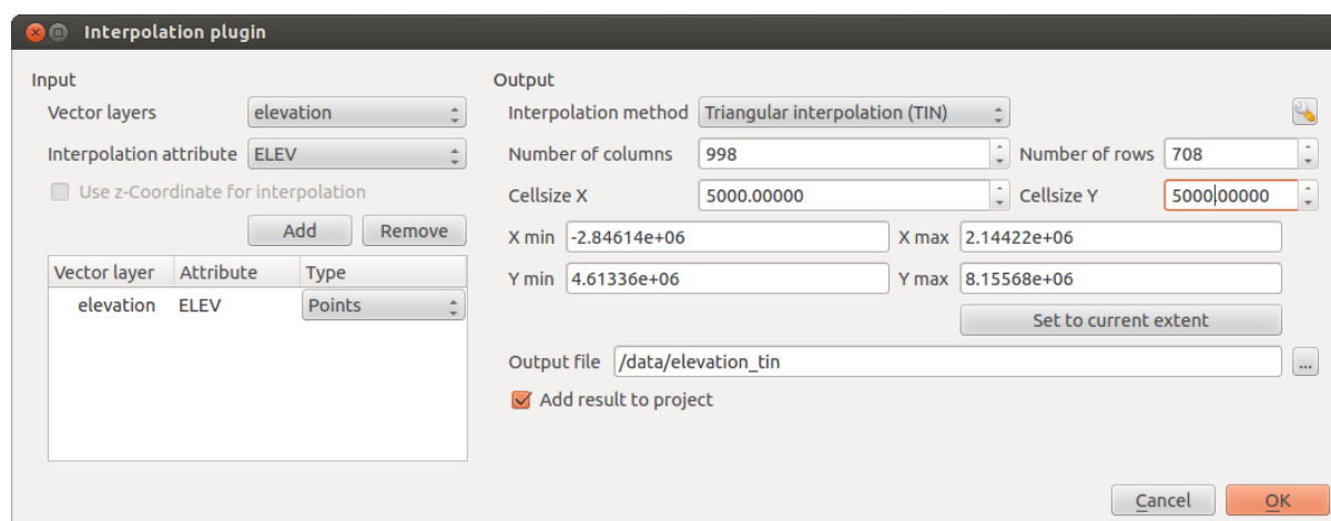
Figure 19.19: Interpolation Plugin
