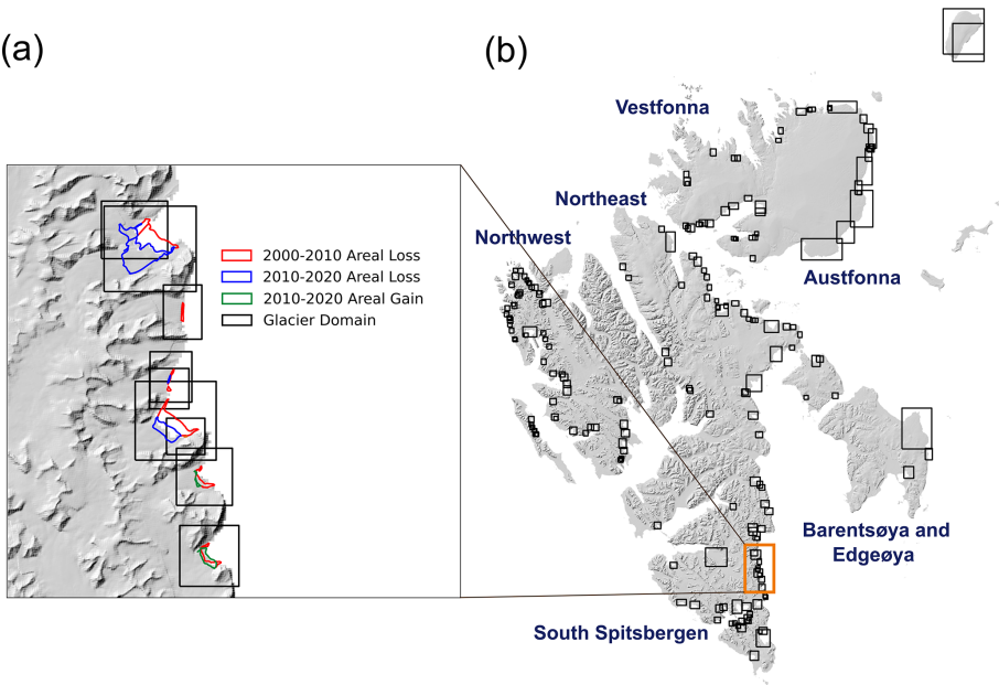
Figure 2. (a) Examples of glacier areal change polygons (coloured outlines) generated in Kochtitzky and Copland (2022) and the glacier domain polygons derived in this study (black boxes). The glacier areal loss during 2000–2010 is denoted as a red polygon, the glacier areal loss during 2010–2020 is denoted as a blue polygon, and the glacier areal gain during 2010–2020 is denoted as a green polygon. (b) The spatial distributions of 220 glacier domains generated in this study (black boxes); the orange box denotes the zoomed-in region shown in panel (a). The background hillshade map is generated from the 50 m resolution Svalbard digital elevation model (DEM) ( https://data.npolar.no/dataset/dce53a47-c726-4845-85c3-a65b46fe2fea , last access: 18 April 2023).
